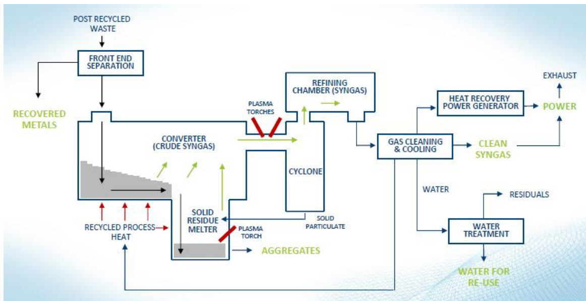
Figure 78 The Plasco gasification system
