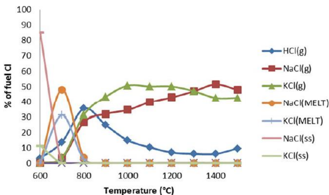
Figure 37 Theoretical distribution of chlorine species in RDF gasification 207
