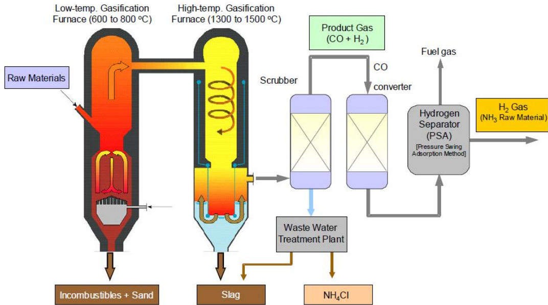
Figure 89 THE EUP process 490
