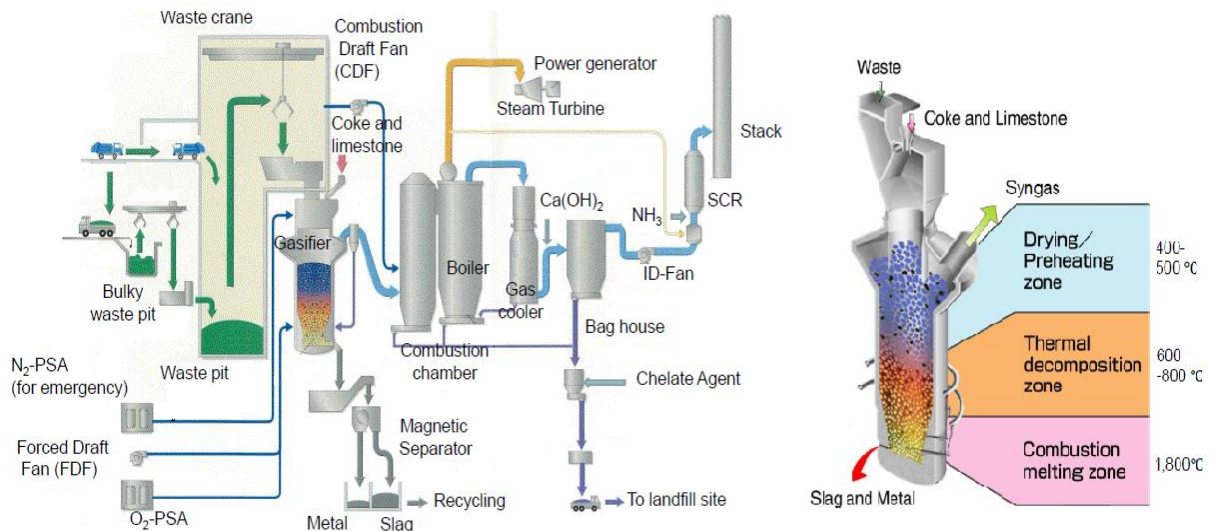
Figure 59 The Nippon Steel & Sumikin Engineering shaft furnace process (adapted from 303 ).
