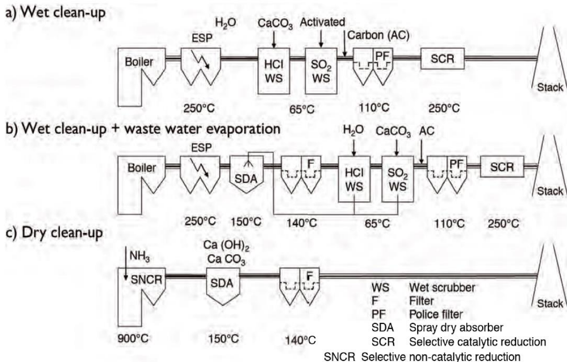
Figure 30 Common configurations for incinerator flue gas cleaning 186
