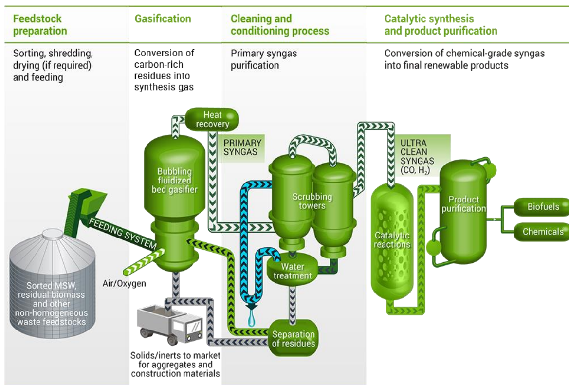
Figure 92 The Enerkem technology 530
