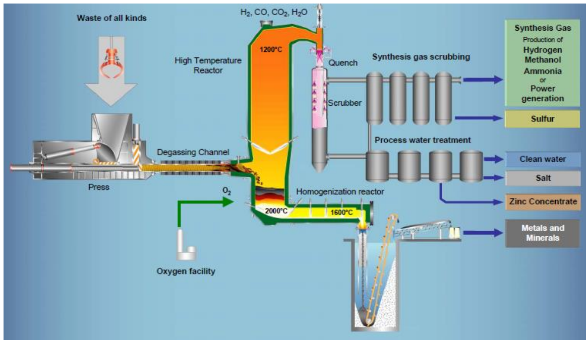
Figure 86 The Thermoselect gasification process 482
