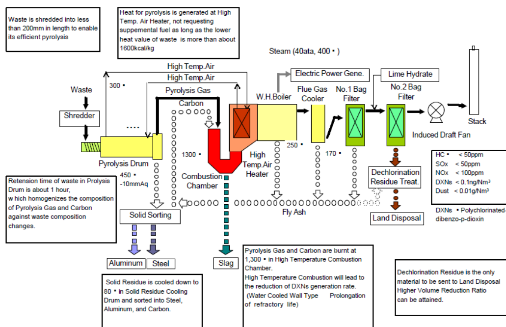
Figure 60 The Mitsui R21 process 306
