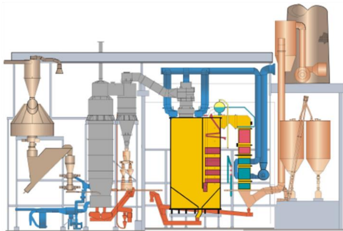
Figure 49 The Stora Enso Ecogas plant at Varkaus, Finland 261, 262 .
